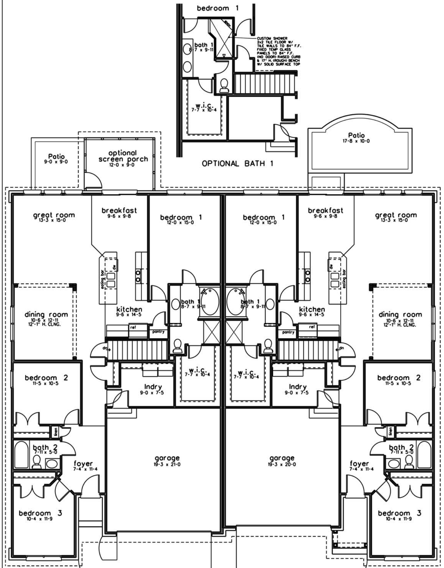
floor plan
